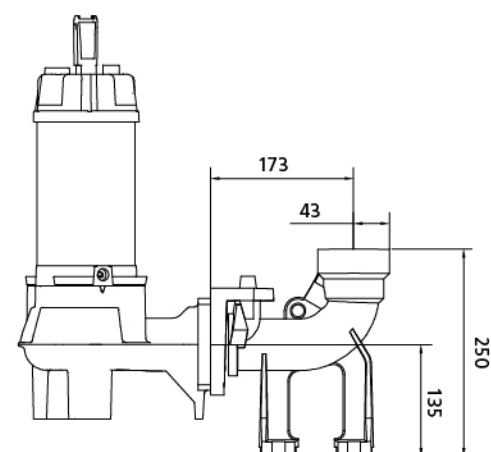
HIPPO with QH coupling foot
